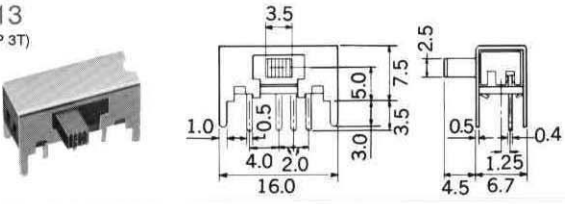
No.MS-333 6P MINIATURE CENTER-OFF SLIDE SWITCH (knob 7m/m) Net Weight : 2.5 gr.
