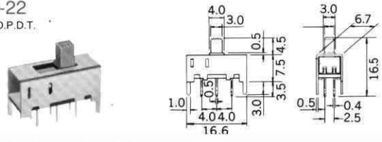
No.MS-292-12 3P MINIATURE SLIDE SWITCH (knob 4.6.7.9m/m) Net Weight : 2.5 gr.
