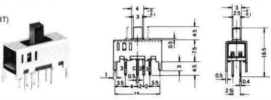
No.MS-033 SLIDE SWITCH (2P 3T) Net Weight : 5 gr.
