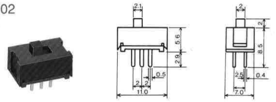
No.MS-7L23 SLIDE SWITCH (2P 3T) Net Weight : 2 gr.
