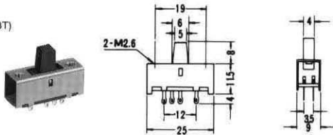
No.MS-7L23 SLIDE SWITCH (2P 3T) Net Weight : 2 gr.
